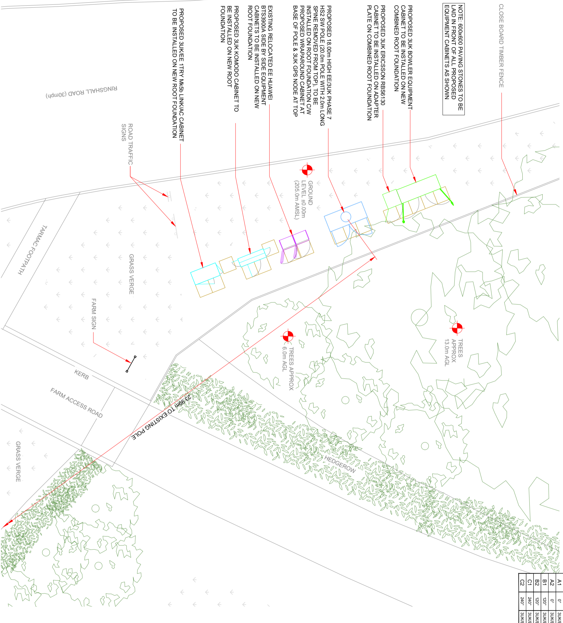
PROPOSED SITE PLAN 1:100 0 2m 4
